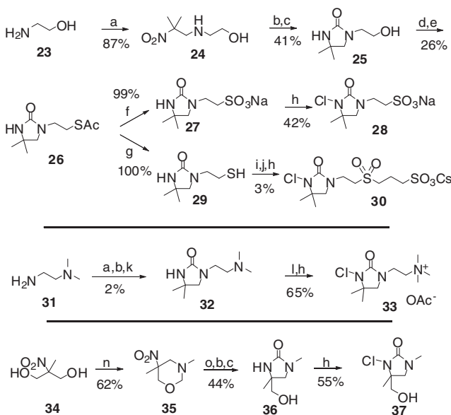
Scheme 5. Reagents and conditions: (a) i -PrOH, \text{CH}_2\text{O} , water, \text{NO}_2\text{CH}(\text{CH}_3)_2 , NaOH, rt, 24 h; (b) Raney Nickel ® , MeOH, \text{H}_2 , rt, 18 h; (c) urea, 200^\circ\text{C} , 1 h; (d) MsCl, pyridine, DCM, rt, 24 h; (e) KSAC, DMF, rt, 18 h; (f) \text{H}_2\text{O}_2 , \text{HCO}_2\text{H} , 0^\circ\text{C} to rt, 16 h; (g) NaOH, MeOH, water, 0^\circ\text{C} to rt, 18 h; (h) t -BuOCl, MeOH, 0^\circ\text{C} , 1 h; (i) propane sultone, \text{Cs}_2\text{CO}_3 , DMF, rt, 18 h; (j) m -CPBA, DCM, rt, 21 h; (k) CDI, DCM, rt, 20 h; (l) MeI, MeOH, rt, 18 h; (m) \text{Ag}_2\text{O} , water, AcOH, rt, 2 h; (n) \text{CH}_2\text{O} , water, \text{CH}_3\text{NH}_2 ; (o) HCl, \text{EtOH} , reflux, 5 h.
