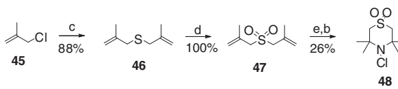
Scheme 6. Reagents and conditions: (a) (i) MeI, DCM, 0^\circ\text{C} , 30 min, (ii) \text{Ag}_2\text{O} , water, rt, 30 min, (iii) HCl, water, rt, 5 min; (b) t -BuOCl, MeOH, 0^\circ\text{C} , 1 h; (c) \text{Na}_2\text{S} , \text{H}_2\text{O} , MeOH, rt to reflux, 8 h; (d) m -CPBA, DCM, 0^\circ\text{C} , 45 min; (e) \text{NH}_4\text{OH} , 60 – 100^\circ\text{C} , 22 h; (f) Raney Nickel ® , methanol, \text{H}_2 , rt, 18 h; (g) acetone, \text{CHCl}_3 , NaOH, rt to reflux, 19 h.
