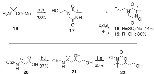
Scheme 4. Reagents and conditions: (a) \text{ClCH}_2\text{COCl} , \text{EtOAc} , \text{H}_2\text{O} , rt, 2 h; (b) ethanolamine, THF; \text{EtOH} , 140^\circ\text{C} , 18 h; (c) DIAD, \text{P}(\text{Ph})_3 , \text{AcSH} , 0^\circ\text{C} to rt, 26 h; (d) \text{HCO}_2\text{H} , \text{H}_2\text{O}_2 , rt, 6 h; (e) t -BuOCl, MeOH, 0^\circ\text{C} to rt, 30 min to 2 h; (h) CDI, THF, rt, 1 h; followed by \text{LiCH}_2\text{CO}_2\text{Et} , -78^\circ\text{C} , 2 h; (i) \text{NaBH}_4 , \text{EtOH} , rt, 3 h; (j) NaH, THF, rt, 4 h.
